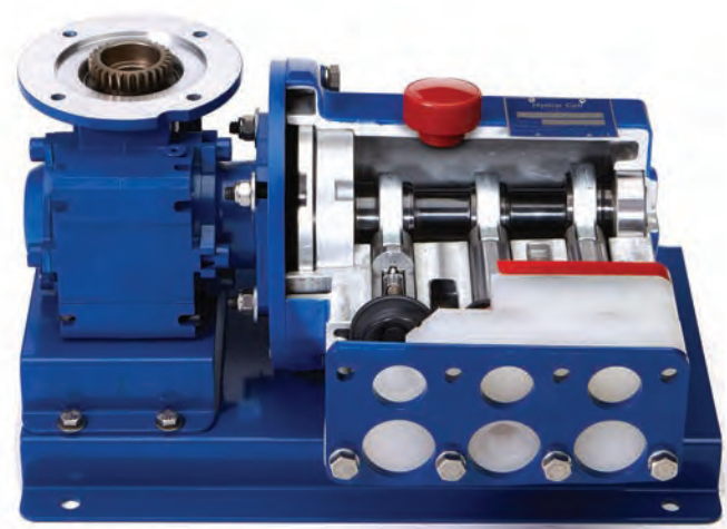
P200 models demonstrate the crank-shaft principle of operation.
