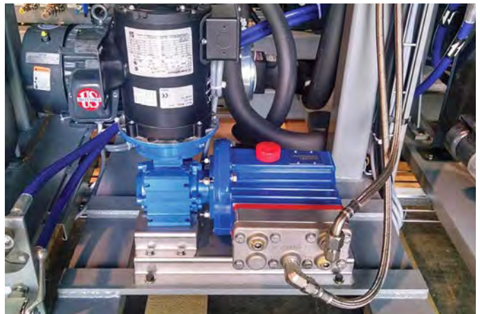
A P200 replaced an external gear pump to deliver a catalyst for polyurethane foam production and doubled volumetric efficiency.
