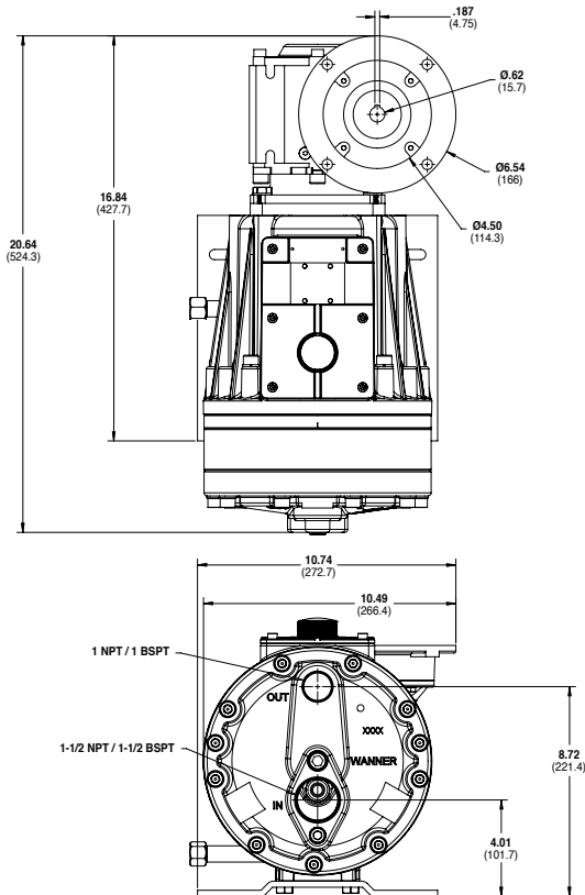
Metallic Pump Heads (NEMA 56C)
