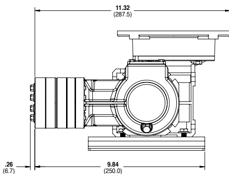
Metallic Pump Heads (NEMA 56C)
